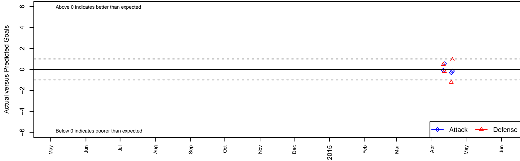
XUnk NSC Impact G99 Dots are actual minus expected GF (blue circles) and GA (red triangles). Blue line is smoothed change in attack strength. Red is smoothed change in defense strength.
